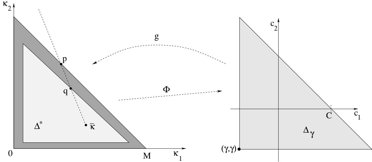
Figure 2: The simplexes \Delta^* = \Delta^{inner} \cup \Delta^{outer} , and \Delta_\gamma .
