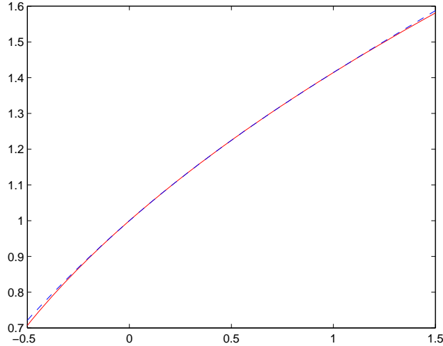
Figure 1: Solid: f(x) , dashed: p_3(x) .
