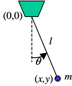
Figure 1: Simple pendulum.
