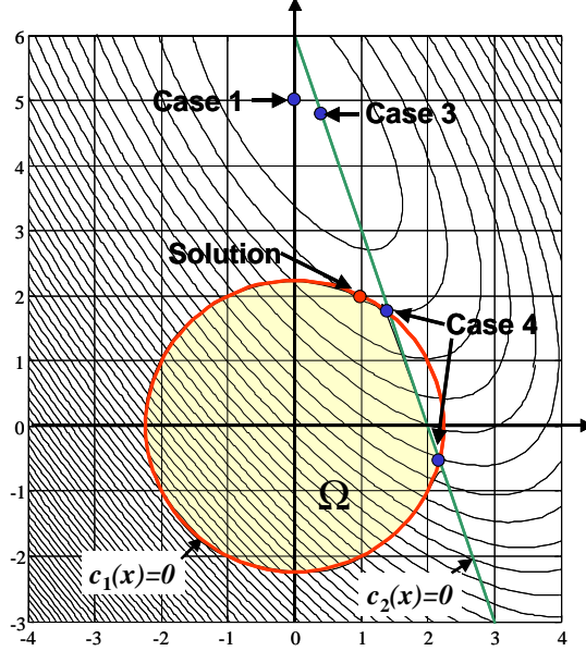
Figure 3: Contours of the objective function and various constraints.
