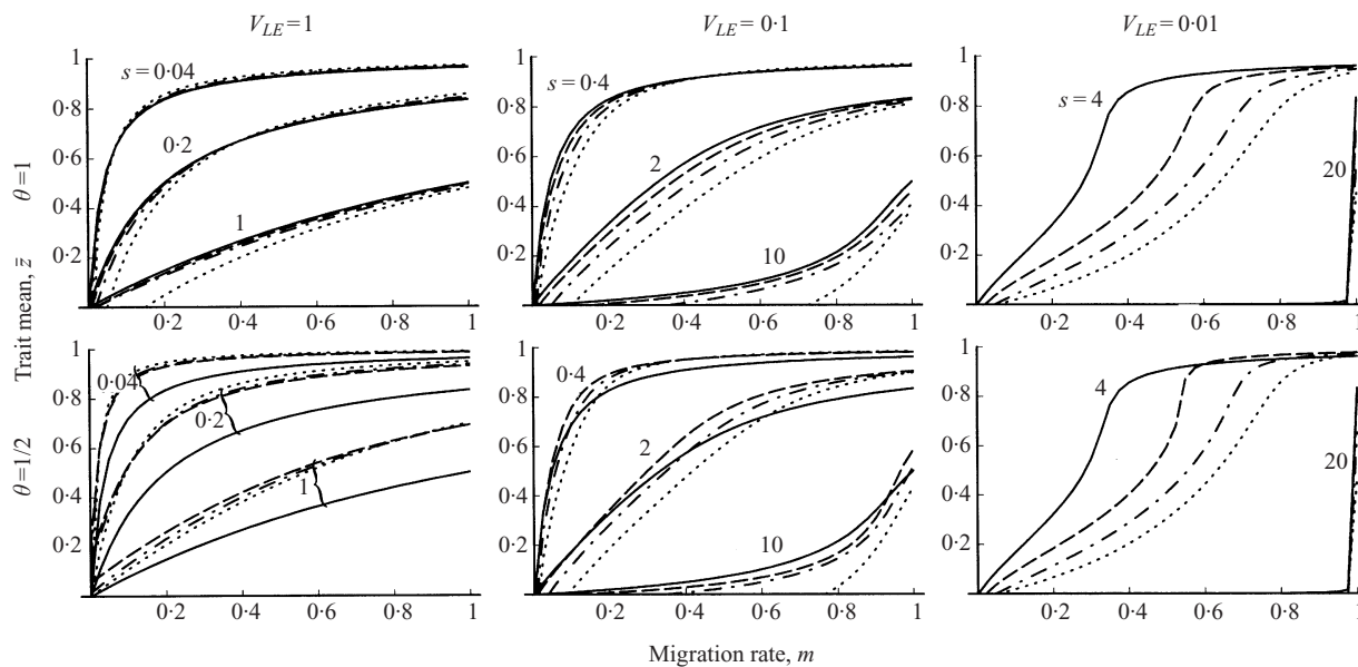
Fig. 3. (a) The mean genotypic value ( z ) as a function of the migration rate ( m ) at equilibrium between migration and stabilizing selection for the infinitesimal model (continuous lines), symmetric model with 5 loci (dashed line), 2 loci (dashed dotted line) and 1 locus (dotted line). Parameters are chosen so that the genetic variances at linkage disequilibrium are the same for the initial local and immigrant population ( \theta = 1 ). The plot is otherwise organized as in Fig. 2a. (b) Same as (a) but with \theta = 1/2 instead of \theta = 1 .
