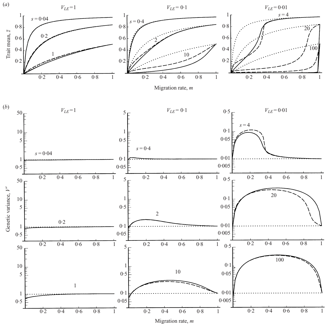
Fig. 2. (a) The mean genotypic value ( \bar{z} ) as a function of the migration rate ( m ) at equilibrium between migration and stabilizing selection for the infinitesimal model (continuous lines), the approximation ignoring deviations from normality (dashed lines) and the approximation ignoring linkage disequilibrium altogether (dotted lines). Each subplot corresponds to different values of V_{LE} (shown in the plot) and each subset of curves within each subplot corresponds to different strengths of selection s . (b) The genetic variance corresponding to each set of curves in (a). Continuous, dashed and dotted lines as in (a).
