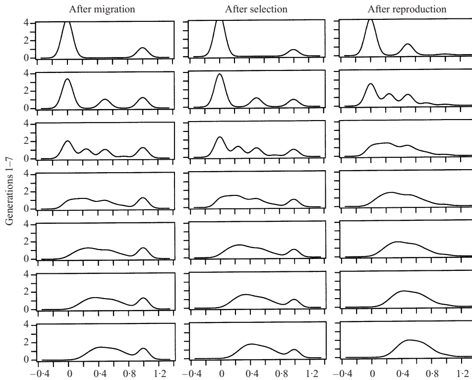
Fig. 1. Iterations of the infinitesimal model for 7 generations (rows 1–7) with z_0 = 0 , z_1 = 1 , s = 1 , m = 0.2 , and V_{LE} = 0.005 , that is, immigrants deviating 14 genetic standard deviations from the optimum. Each subplot shows the distribution of genotypic values ( z ) after migration (left-hand column), selection (middle column) and reproduction (right-hand column). F1 and F2 crosses and backcrosses with the local and immigrant population can be seen as clear modes in the distribution in generations 2 and 3. The parameter values are chosen for illustrative purposes. It might be noted that the distribution for the above parameter values eventually (after about 85 generations by the criteria in the main text) reached an equilibrium at which \bar{z} = 0.974 and \text{Var}(z) = 0.00506 , that is, very little linkage disequilibrium.
