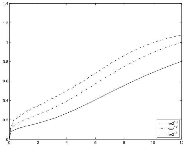
FIG. 3.4. Plot of \|u(t) - u^n(t)\|_{H^1} / \|u(t)\|_{H^1} in the two peakon case of Figure 3.3.
