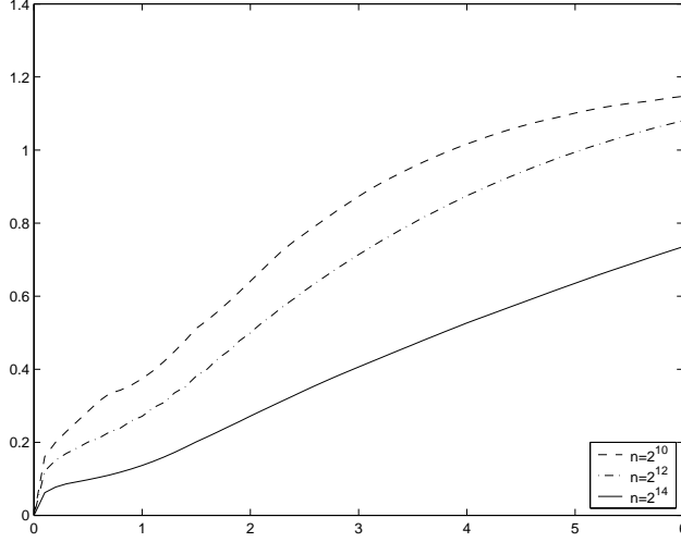
FIG. 3.2. Plot of \|u(t) - u^n(t)\|_{H^1} / \|u(t)\|_{H^1} in the one peakon case of Figure 3.1.
