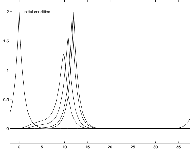
FIG. 3.1. Periodic single peakon. The initial condition is given by u(x, 0) = 2e^{-|x|} and period a = 40 . The computed solutions are shown at time t = 6 for (from left to right) n = 2^{10} , n = 2^{12} , n = 2^{14} together with the exact solution (at the far right).
