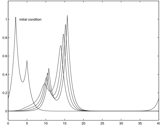
FIG. 3.3. Two peakon case. The initial condition is the periodized version of 2e^{-|x-2|} + e^{-|x-5|} . The computed solutions are shown at time t = 12 for (from left to right) n = 2^{10} , n = 2^{12} , n = 2^{14} together with the exact solution (at the far right).
