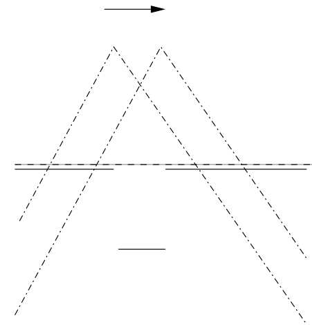
Figure 6: Rotating a Broken Loop
