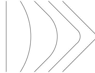
Figure 2: Interpolation I: Piecewise-Smooth
