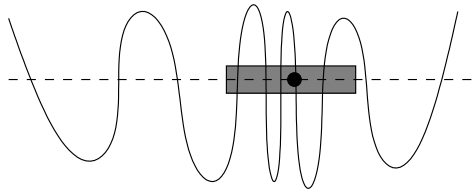
Figure 4: A Loop Close to the Zero Loop
