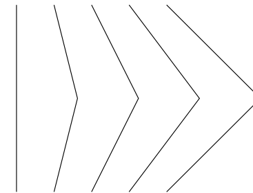
Figure 3: Interpolation II: Piecewise-Smooth and Bounded
