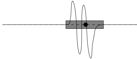
Figure 5: Applying a Bump Function
