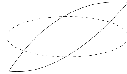
Figure 7: The Loop \alpha_0
