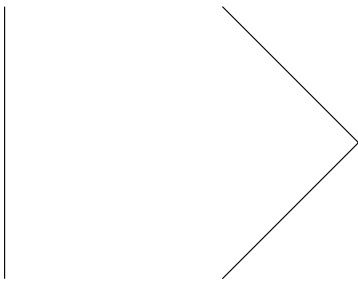
Figure 1: Close-up of two paths
