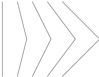
Figure 3: Interpolation II: Piecewise-Smooth and Bounded
