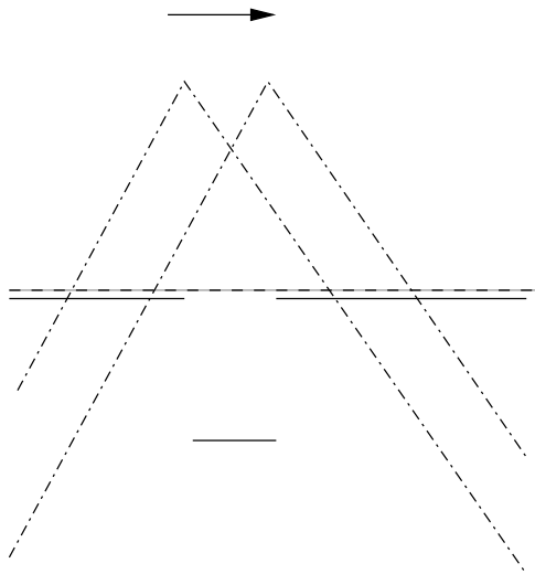
Figure 6: Rotating a Broken Loop
