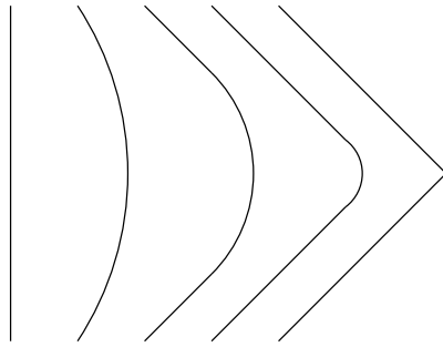
Figure 2: Interpolation I: Piecewise-Smooth
