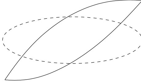
Figure 7: The Loop \alpha_0
