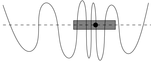
Figure 4: A Loop Close to the Zero Loop
