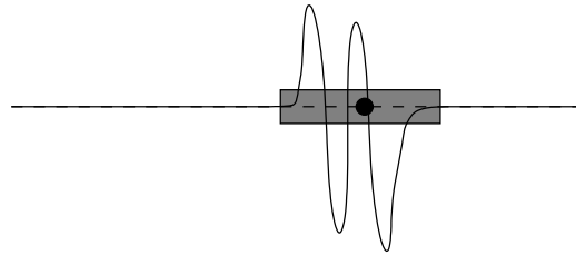
Figure 5: Applying a Bump Function
