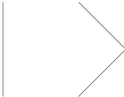
Figure 1: Close-up of two paths
