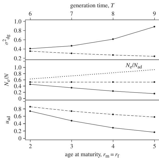
Figure 2. Effects of age at maturity, r , on the genetic drift per time step, \sigma_{\text{dg}}^2 , the ratio of effective population size to census (total) population size, N_e/N , and the proportion of adults at stable stage structure, u_{\text{ad}} , in populations with different levels of juvenile survival. Annual survival probability of prereproductive individuals, s_{\text{ym}} = s_{\text{yf}} , is equal to 0.5 (solid lines) and 1 (dashed lines). In the middle panel, the dotted line shows the ratio N_e/N_{\text{ad}} , where N_{\text{ad}} is the adult population size (as opposed to the total population size used in the ratio N_e/N represented by the solid and dashed lines). Variance in annual male mating success is equal to 2, the sex ratio, q , is equal to 0.5, and the expected number of offspring is adjusted to maintain a growth rate, \lambda , of 1.
