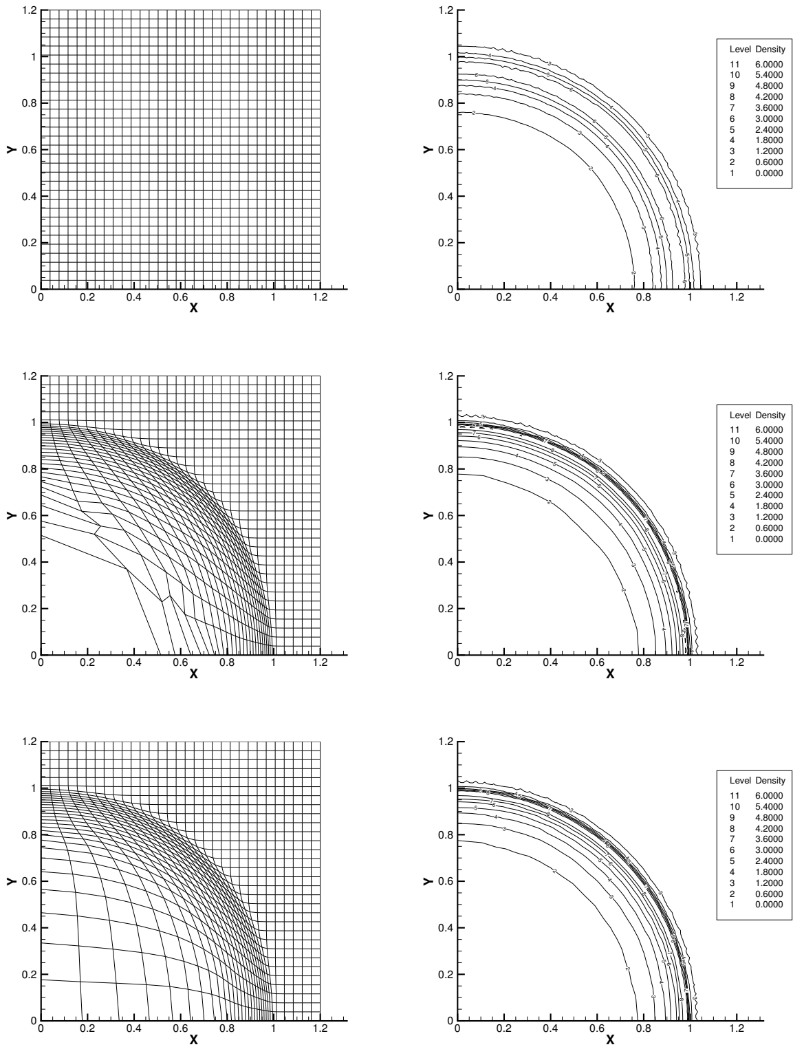
Fig. 10. Sedov problem — Quadrilateral Mesh. Mesh (left), and density isolines (right) at t = 1.0 — Eulerian regime (top), Lagrangian regime (middle), ALE regime (bottom).
