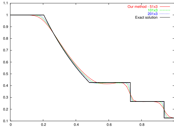
Fig. 7. Convergence for Sod problem: density at t = 0.25 for N_x = 50, 100, 200 .
