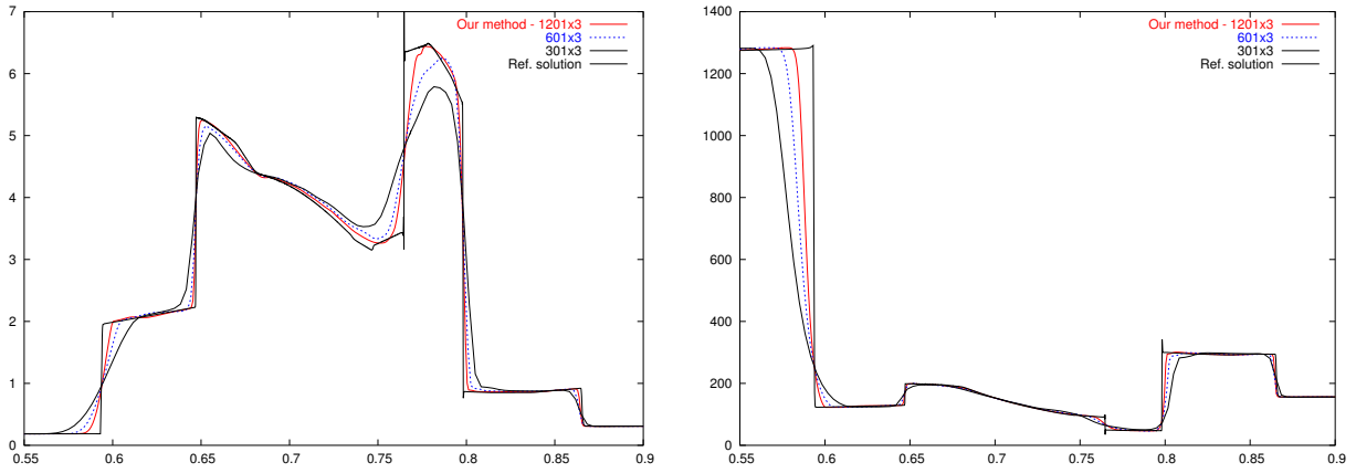
Fig. 8. Convergence for Woodward-Colella Blast Wave Problem. Density (zoom) — left, and specific internal energy (zoom) — right at t = 0.038 , N_x = 300, 600, 1200 .
