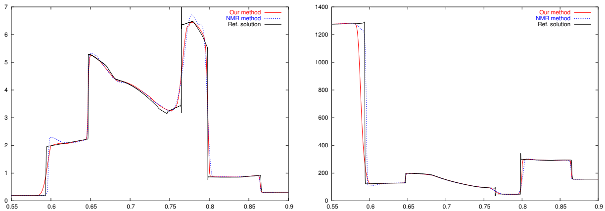
Fig. 5. Woodward-Colella Blast Wave Problem. Comparison of the NMR method and the new method: density (zoom) — left, and specific internal energy (zoom) — right at t = 0.038 , N_x = 1200 .
