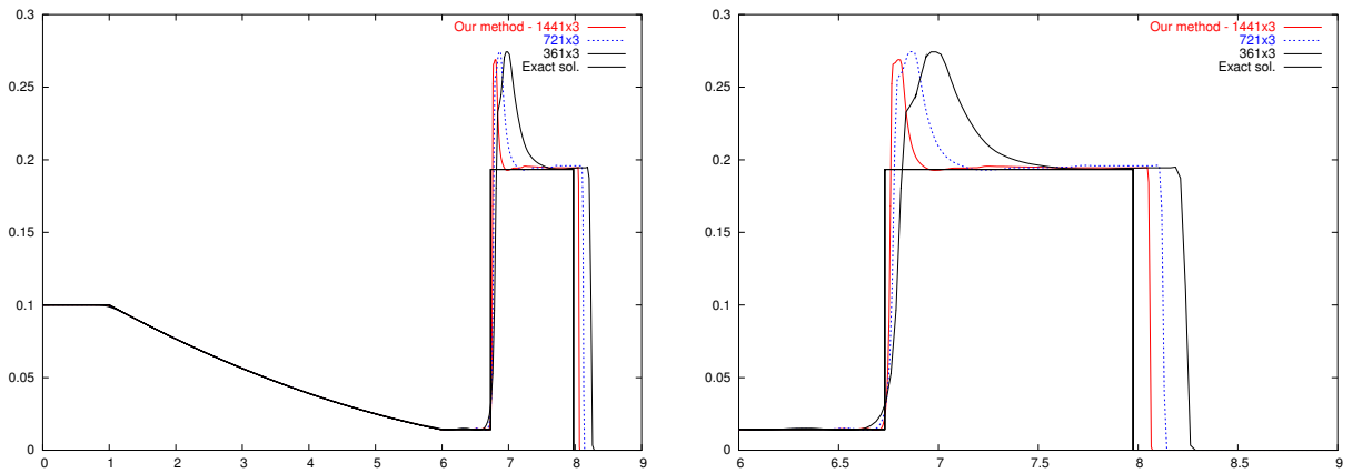
Fig. 9. Specific internal energy for LeBlanc shock tube problem at t = 6.0 , N_x = 360, 720, 1440 : entire computational domain — left, zoom — right.
