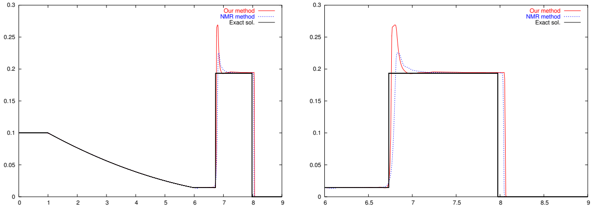
Fig. 6. LeBlanc shock tube problem. Comparison of the NMR method and the new method — specific internal energy at t = 6.0 , N_x = 1440 : entire computational domain — left, zoom — right.
