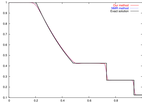
Fig. 4. Sod test problem. Comparison of our new method and the NRM method: density at t = 0.25 , N_x = 200 .
