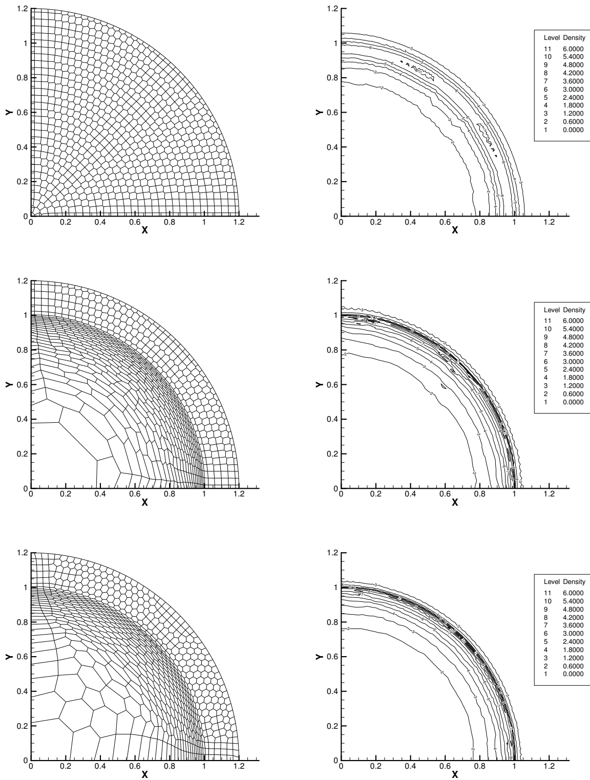
Fig. 12. Sedov problem — Polygonal Mesh. Mesh (left), and density isolines (right) at t = 1.0 — Eulerian regime (top), Lagrangian regime (middle), ALE regime (bottom).
