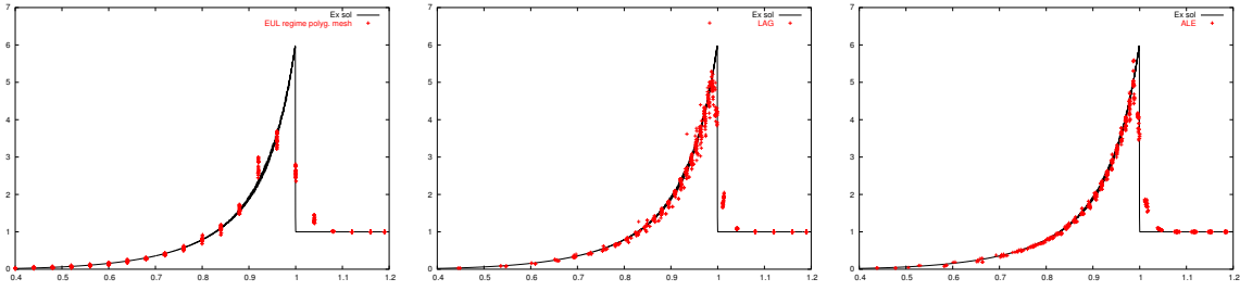
Fig. 13. Sedov problem — Polygonal Mesh. Density at t = 1.0 as a function of the radius (solid line exact solution) — Eulerian regime (left), Lagrangian regime (middle), ALE regime (right).
