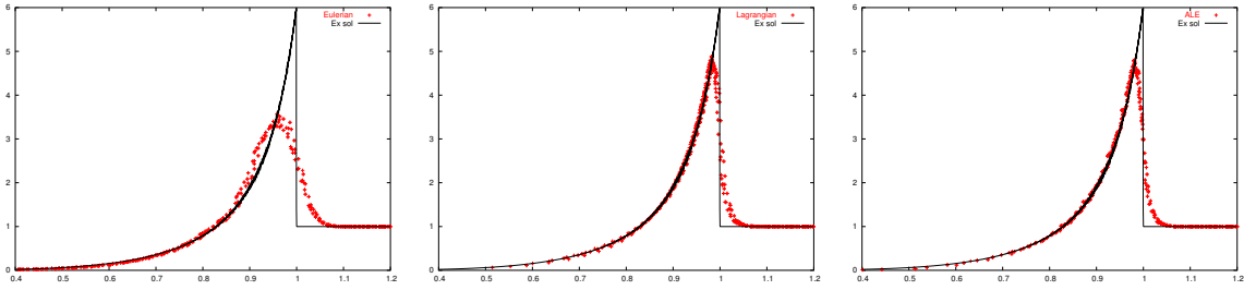
Fig. 11. Sedov problem — Quadrilateral Mesh. Density at t = 1.0 as a function of the radius (solid line exact solution) — Eulerian regime (left), Lagrangian regime (middle), ALE regime (right).
