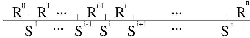
FIGURE 3.1. Ordering of regular and singular layers.
