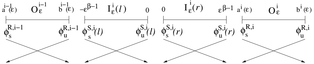
FIGURE 5.1. Notations for the initial data \phi_u^{R,i} , etc. The solutions passing through them decay exponentially in the direction indicated by the arrows.
