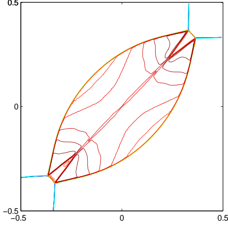
Figure 4.4: [S_{12}^+ S_{23}^- S_{34}^+ S_{41}^-] . The initial data are \rho_1=1, u_1=-0.5612, v_1=-0.5612, p_1=0.7; \rho_2=2.5, u_2=0.5612, v_2=-0.5612, p_2=2.8; \rho_3=1, u_3=0.5612, v_3=0.5612, p_3=0.7; \rho_4=2.5, u_4=-0.5612, v_4=0.5612, p_4=2.8 . The meshes are 200 \times 200 . The output time is t=0.25 . The monitor function is \omega = \sqrt{1+0.05|\nabla e|^2} .
