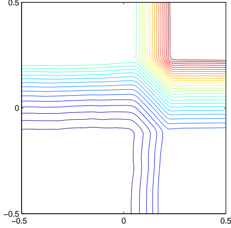
Figure 4.14: [R_{12}^+ R_{23}^+ R_{34}^- R_{41}^-] . The initial data are \rho_1 = 1.0, u_1 = 0.0, v_1 = 0.0, p_1 = 1.0 ; \rho_2 = 0.5179, u_2 = -0.7259, v_2 = 0.0, p_2 = 0.4 ; \rho_3 = 0.1072, u_3 = -0.7259, v_3 = -1.4045, p_3 = 0.0439 ; \rho_4 = 0.2579, u_4 = 0.0, v_4 = -1.4045, p_4 = 0.15 . The mesh cells are 100 \times 100 . The output time is t = 0.2 . The monitor function is \omega = \sqrt{1 + 100(|\bar{\nabla}u|^2 + |\bar{\nabla}v|^2 + |\bar{\nabla}\rho|^2)} .
