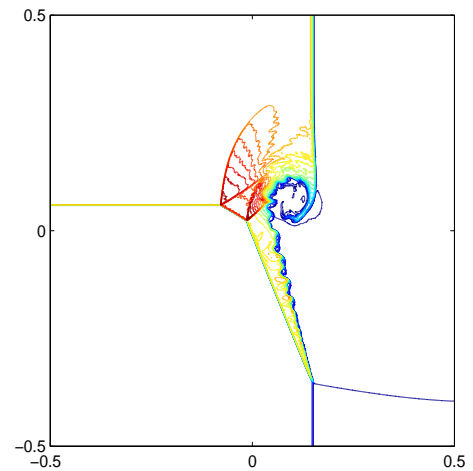
Figure 4.13: [J_{12}^- S_{23}^- J_{34}^+ S_{41}^+] . The initial data are \rho_1 = 2.04, u_1 = 1.0, v_1 = -1.0, p_1 = 15.0; \rho_2 = 15.0, u_2 = 1.0, v_2 = 0.0, p_2 = 15.0; \rho_3 = 4.4022, u_3 = 1.0, v_3 = 2.4444, p_3 = 2.0; \rho_4 = 0.5870, u_4 = 1.0, v_4 = 2.9558, p_4 = 2.0 . The mesh cells are 1200 \times 1200 . The output time is t=0.15 . The monitor function is \omega = \sqrt{1+0.01(|\nabla \rho|^2 + |\nabla u|^2 + |\nabla v|^2)} .
