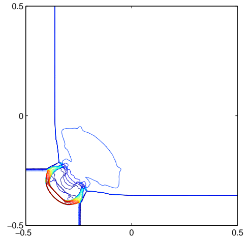
Figure 4.11: [S_{12}^- J_{23}^- J_{34}^+ S_{41}^+] . The initial data are \rho_1 = 7.039, u_1 = -2.037, v_1 = -2.037, p_1 = 30.0, \rho_2 = 1.4, u_2 = 2.037, v_2 = -2.037, p_2 = 1.0, \rho_3 = 7.039, u_3 = -2.037, v_3 = -2.037, p_3 = 1.0, \rho_4 = 1.4, u_4 = -2.037, v_4 = 2.037, p_4 = 1.0 . The mesh cells are 400 \times 400 . The output time is t=0.119 . The monitor function is \omega = \sqrt{1+5.0(|\nabla \rho|^2 + |\nabla u|^2 + |\nabla v|^2)} .
