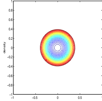
(a) Contour lines for density
