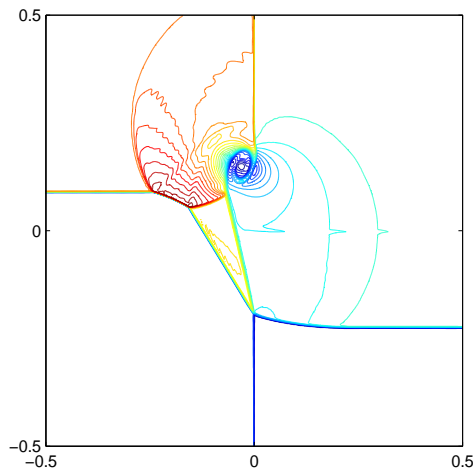
Figure 4.12: [J_{12}^- S_{23}^- J_{34}^+ S_{41}^+] . The initial data are \rho_1 = 1.0, u_1 = 0.0, v_1 = 0.0, p_1 = 1.0; \rho_2 = 1.4, u_2 = 0.0, v_2 = 1.0, p_2 = 1.0; \rho_3 = 0.7, u_3 = 0.0, v_3 = 1.6742, p_3 = 0.3636; \rho_4 = 0.5, u_4 = 0.0, v_4 = 0.7978, p_4 = 0.3636 . The mesh cells are 100 \times 100 . The output time is t=0.28 . The monitor function is \omega = \sqrt{1+40.0(|\nabla \rho|^2 + |\nabla u|^2 + |\nabla v|^2)} .
