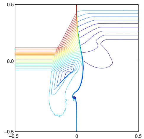
Figure 4.19: [J_{12}^+ R_{23}^+ J_{34}^+ R_{41}^-] . The initial data are \rho_1 = 1.0, u_1 = 0.0, v_1 = 0.3, p_1 = 1.0 ; \rho_2 = 2.0, u_2 = 0.0, v_2 = -0.3, p_2 = 1.0 ; \rho_3 = 1.039, u_3 = 0.0, v_3 = -0.8133, p_3 = 0.4 ; \rho_4 = 0.5197, u_4 = 0.0, v_4 = -0.4259, p_4 = 0.4 . The mesh cells are 800 \times 800 . The output time is t = 0.3 . The monitor function is \omega = \sqrt{1 + 1.0(|\nabla u|^2 + |\nabla v|^2 + |\nabla \rho|^2)} .
