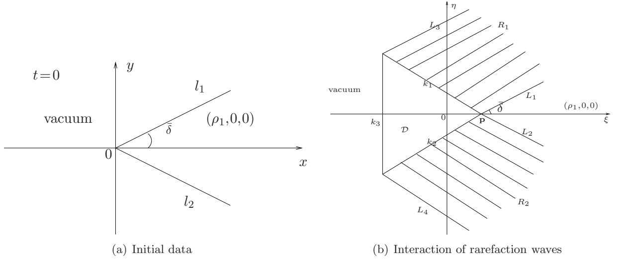
Figure A.1: The expansion of wedge of gas.
