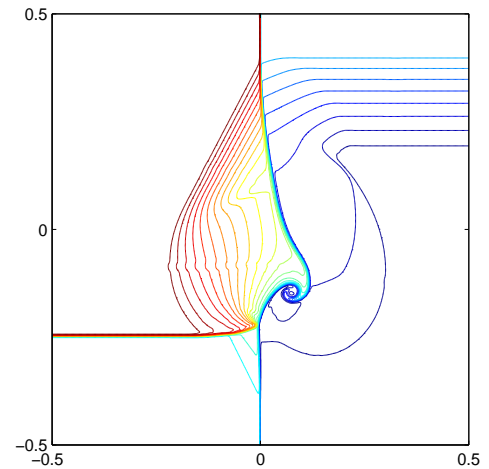
Figure 4.25: [J_{12}^+ S_{23}^- J_{34}^- R_{41}^+] . The initial data are \rho_1 = 1.0, u_1 = 0.0, v_1 = 0.3, p_1 = 1.0 ; \rho_2 = 2.0, u_2 = 0.0, v_2 = -0.3, p_2 = 1.0 ; \rho_3 = 1.0625, u_3 = 0.0, v_3 = 0.2145, p_3 = 0.4 ; \rho_4 = 0.5179, u_4 = 0.0, v_4 = -0.4259, p_4 = 0.4 . The mesh cells are 200 \times 200 . The output time is t = 0.26 . The monitor function is \omega = \sqrt{1 + 50(|\nabla u|^2 + |\nabla v|^2) + 10|\nabla \rho|^2} .
