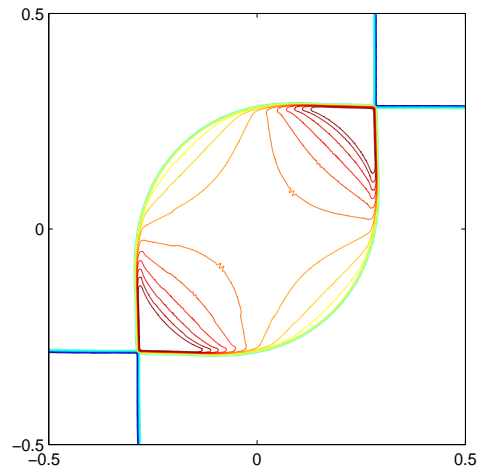
Figure 4.3: [S_{12}^+ S_{23}^- S_{34}^+ S_{41}^-] . The initial data are \rho_1 = 1 , u_1 = -0.189970 , v_1 = -0.189970 , p_1 = 1.4 ; \rho_2 = 1.3 , u_2 = 0.189970 , v_2 = -0.189970 , p_2 = 2.025532 ; \rho_3 = 1 , u_3 = 0.189970 , v_3 = 0.189970 , p_3 = 1.4 ; \rho_4 = 1.3 , u_4 = -0.189970 , v_4 = 0.189970 , p_4 = 2.025532 . The output time is t = 0.2 . The meshes are 200 \times 200 . The monitor function is \omega = \sqrt{1 + 5|\nabla e|^2} .
