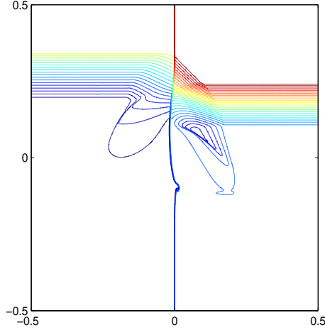
Figure 4.20: [J_{12}^+ R_{23}^+ J_{34}^- R_{41}^-] . The initial data are d1 = 1.5, u1=0.0, v1=0.0, p1=2.0 ; d2=1.2, u2=0.0, v2=0.4, p2=2.0 ; d3=0.731408, u3=0.0, v3=-0.32, p3=1.0 ; d4=0.91426, u4=0.0, v4=-0.64403, p4=1.0 . The mesh cells are 800 \times 800 . The output time is t = 0.18 . The monitor function is \omega = \sqrt{1+1.0(|\bar{\nabla}u|^2+|\bar{\nabla}v|^2+|\bar{\nabla}\rho|^2)} .
