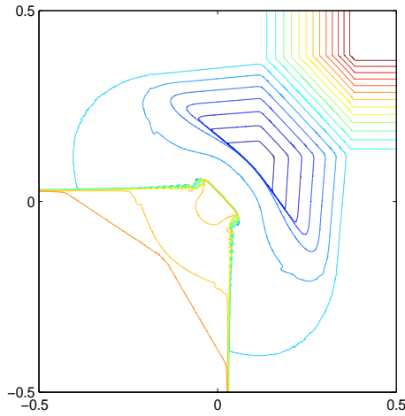
Figure 4.16: [R_{12}^+ J_{23}^+ J_{34}^- R_{41}^-] . The initial data are \rho_1 = 1.0, u_1 = 0.1, v_1 = 0.1, p_1 = 1.0 ; \rho_2 = 0.5197, u_2 = -0.6259, v_2 = 0.1, p_2 = 0.4 ; \rho_3 = 0.8, u_3 = 0.1, v_3 = 0.1, p_3 = 0.4 ; \rho_4 = 0.5197, u_4 = 0.1, v_4 = -0.6259, p_4 = 0.4 . The mesh cells are 800 \times 800 . The output time is t = 0.3 . The monitor function is \omega = \sqrt{1 + 200(|\nabla u|^2 + |\nabla v|^2 + |\nabla \rho|^2)} .
