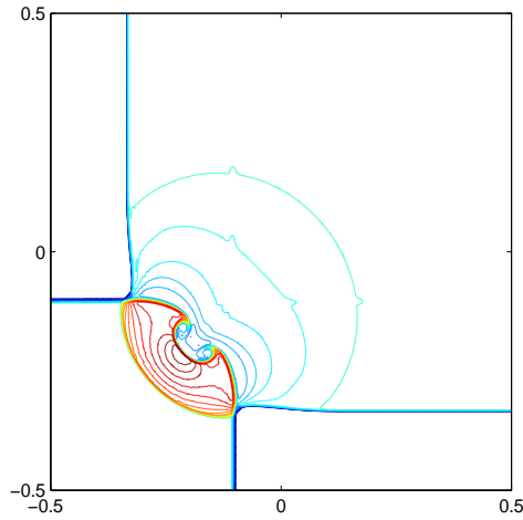
Figure 4.10: [S_{12}^- J_{23}^- J_{34}^+ S_{41}^+] . The initial data are \rho_1=1.0, u_1=-0.3638, v_1=-0.3638, p_1=1.0, \rho_2=0.5313, u_2=0.3638, v_2=-0.3638, p_2=0.4, \rho_3=1.0, u_3=-0.3638, v_3=-0.3638, p_3=0.4, \rho_4=0.5313, u_4=-0.3638, v_4=0.3638, p_4=0.4 . The mesh cells are 200 \times 200 . The output time is t=0.28 . The monitor function is \omega = \sqrt{1+50(|\nabla \rho|^2 + |\nabla u|^2 + |\nabla v|^2)} .
