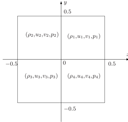
Figure 4.1: The initial data for the 2D Riemann problem.
