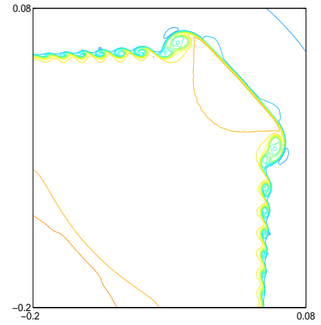
Figure 4.17: Local enlargement of Figure 4.16 for vortices.
