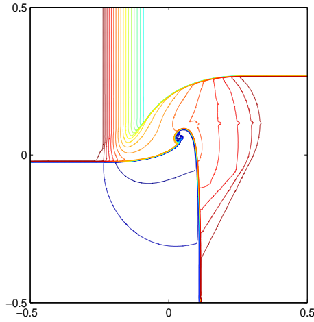
Figure 4.22: [R_{12}^- J_{23}^+ J_{34}^+ S_{41}^-] . The initial data are d1 = 1.5, u1 = 0.5, v1 = -0.1, p1 = 0.8 ; d2 = 2.7824, u2 = -0.06828, v2 = -0.1, p2 = 1.9 ; d3 = 0.9, u3 = 0.5, v3 = -0.1, p3 = 1.9 ; d4 = 2.7313, u4 = 0.5, v4 = 0.4750, p4 = 1.9 . The mesh cells are 400 \times 400 . The output time is t = 0.2 . The monitor function is \omega = \sqrt{1 + 50(|\nabla u|^2 + |\nabla v|^2) + 10|\nabla \rho|^2} .
