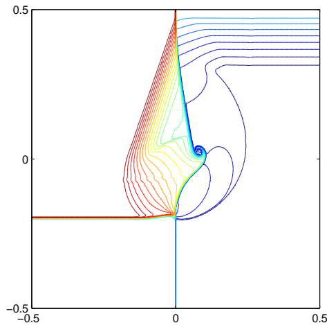
Figure 4.24: [J_{12}^+ S_{23}^- J_{34}^+ R_{41}^+] . The initial data are d1 = 1.0, u1 = 0.0, v1 = 1.0, p1 = 1.0 ; d2 = 2.0, u2 = 0.0, v2 = -0.3, p2 = 1.0 ; d3 = 1.0625, u3 = 0.0, v3 = 0.2145, p3 = 0.4 ; d4 = 0.5179, u4 = 0.0, v4 = 0.2741, p4 = 0.4 . The mesh cells are 200 \times 200 . The output time is t = 0.2 . The monitor function is \omega = \sqrt{1 + 50(|\nabla u|^2 + |\nabla v|^2) + 10|\nabla \rho|^2} .
