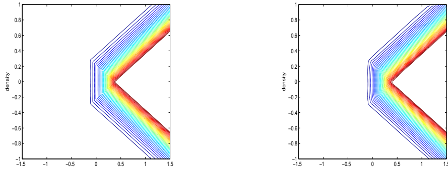
Figure 3.1: The dam collapse problem. The left is the exact solution and the right is the numerical solution with 160 \times 160 adaptive meshes at t=0.2 and the monitor function \omega = \sqrt{1+10|\bar{\nabla}\rho|^2} .
