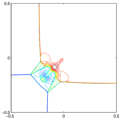
Figure 4.2: [S_{12}^+ S_{23}^+ S_{34}^- S_{41}^-] . The initial data are \rho_1 = 1.5 , u_1 = 0 , v_1 = 0 , p_1 = 1.5 ; \rho_2 = 0.5323 , u_2 = 1.206 , v_2 = 0 , p_2 = 0.3 ; \rho_3 = 0.138 , u_3 = 1.206 , v_3 = 1.206 , p_3 = 0.029 ; \rho_4 = 0.5323 , u_4 = 0 , v_4 = 1.206 , p_4 = 0.3 . The meshes are 200 \times 200 . The output time is t = 0.35 . The monitor function is \omega = \sqrt{1 + 0.01|\nabla e|^2} .
