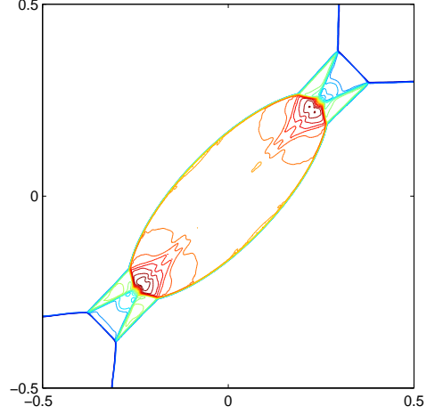
Figure 4.5: [S_{12}^+ S_{23}^- S_{34}^+ S_{41}^-] . The initial data are \rho_1=1.4, u_1=-4.125, v_1=-4.125, p_1=1; \rho_2=8, u_2=4.125, v_2=-4.125, p_2=116.5; \rho_3=1.4, u_3=4.125, v_3=4.125, p_3=1; \rho_4=8, u_4=-4.125, v_4=4.125, p_4=116.5 . The meshes are 100 \times 100 . The output time is t=0.05 . The monitor function is \omega = \sqrt{1+0.05|\nabla e|^2} .
