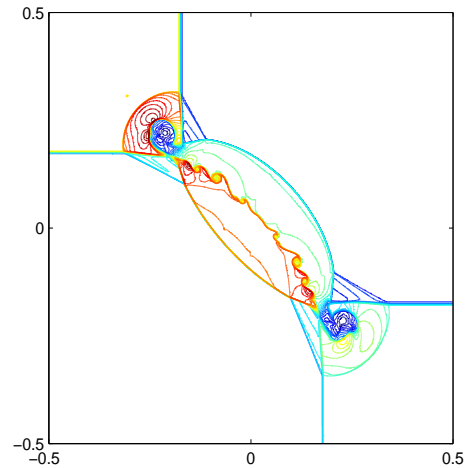
Figure 4.7: [J_{12}^- J_{23}^+ J_{34}^- J_{41}^+] . The initial data are \rho_1 = 0.5, u_1 = -0.5, v_1 = -0.5, p_1 = 0.15 ; \rho_2 = 1.5, u_2 = -0.5, v_2 = 0.5, p_2 = 0.15 ; \rho_3 = 0.75, u_3 = 0.5, v_3 = 0.5, p_3 = 0.15 ; \rho_4 = 1.0, u_4 = 0.5, v_4 = -0.5, p_4 = 0.15 . The meshes are 800 \times 800 . The output time is t = 0.35 . The monitor function is \omega = \sqrt{1 + 5(|\bar{\nabla}\rho|^2 + |\bar{\nabla}u|^2 + |\bar{\nabla}v|^2)} .
