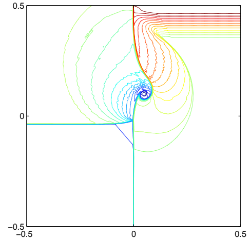
Figure 4.23: [J_{12}^- S_{23}^- J_{34}^- R_{41}^-] . The initial data are \rho_1 = 1.2, u_1 = 0.0, v_1 = 0.6, p_1 = 0.8 ; \rho_2 = 0.9, u_2 = 0.0, v_2 = 0.8, p_2 = 0.8 ; \rho_3 = 0.645283, u_3 = 0.0, v_3 = 1.162738, p_3 = 0.5 ; \rho_4 = 0.857791, u_4 = 0.0, v_4 = 0.286315, p_4 = 0.5 . The mesh cells are 200 \times 200 . The output time is t = 0.3 . The monitor function is \omega = \sqrt{1 + 50(|\nabla u|^2 + |\nabla v|^2) + 10|\nabla \rho|^2} .
