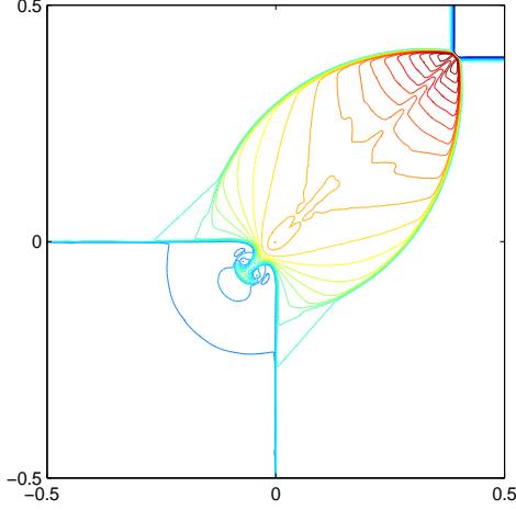
Figure 4.8: [S_{12}^+ J_{23}^- J_{34}^+ S_{41}^-] . The initial data are \rho_1 = 0.5313, u_1 = 0.0, v_1 = 0.0, p_1 = 0.4 ; \rho_2 = 1.0, u_2 = 0.7267, v_2 = 0.0, p_2 = 1.0 ; \rho_3 = 0.8, u_3 = 0.0, v_3 = 0.0, p_3 = 1.0 ; \rho_4 = 1.0, u_4 = 0.0, v_4 = 0.7276, p_4 = 1.0 . The meshes are 100 \times 100 . The output time is t = 0.25 . The monitor function is \omega = \sqrt{1 + 50(|\nabla u|^2 + |\nabla v|^2) + 10|\nabla \rho|^2} .
