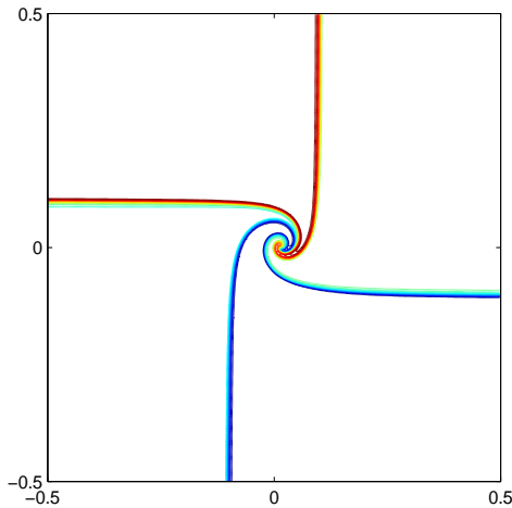
Figure 4.6: [J_{12}^- J_{23}^- J_{34}^- J_{41}^-] . The initial data are \rho_1 = 0.1, u_1 = 0.5, v_1 = -0.5, p_1 = 10.0 ; \rho_2 = 0.15, u_2 = 0.5, v_2 = 0.5, p_2 = 10.0 ; \rho_3 = 0.09, u_3 = -0.5, v_3 = 0.5, p_3 = 10.0 ; \rho_4 = 0.05, u_4 = -0.5, v_4 = -0.5, p_4 = 10.0 . The meshes are 100 \times 100 . The output time is t = 0.2 . The monitor function is \omega = \sqrt{1 + 10(|\bar{\nabla}\rho|^2 + |\bar{\nabla}u|^2 + |\bar{\nabla}v|^2)} .
