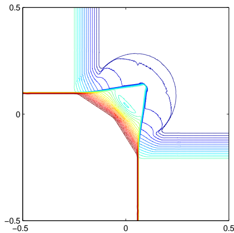
Figure 4.18: [R_{12}^- J_{23}^+ J_{34}^- R_{41}^+] . The initial data are \rho_1 = 0.5686, u_1 = 0.3, v_1 = 0.5, p_1 = 0.3302 ; \rho_2 = 1.0, u_2 = -0.244, v_2 = 0.5, p_2 = 0.7279 ; \rho_3 = 1.5, u_3 = 0.3, v_3 = 0.5, p_3 = 0.7279 ; \rho_4 = 1.0, u_4 = 0.3, v_4 = -0.0389, p_4 = 0.7279 . The mesh cells are 100 \times 100 . The output time is t = 0.2 . The monitor function is \omega = \sqrt{1 + 200(|\nabla u|^2 + |\nabla v|^2 + |\nabla \rho|^2)} .
