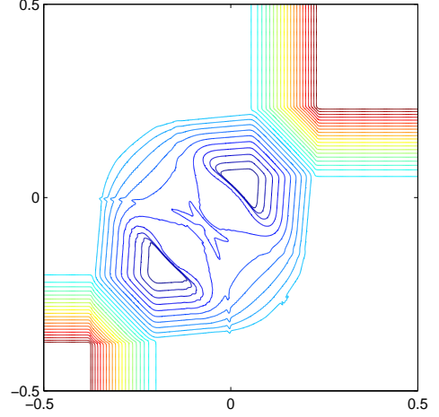
Figure 4.15: [R_{12}^+ R_{23}^- R_{34}^+ R_{41}^-] . The initial data are \rho_1 = 1.0, u_1 = 0.0, v_1 = 0.0, p_1 = 1.0 ; \rho_2 = 0.5197, u_2 = -0.7259, v_2 = 0.0, p_2 = 0.4 ; \rho_3 = 1.0, u_3 = -0.7259, v_3 = -0.7259, p_3 = 1.0 ; \rho_4 = 0.5179, u_4 = 0.0, v_4 = -0.7259, p_4 = 0.4 . The mesh cells are 100 \times 100 . The output time is t = 0.2 . The monitor function is \omega = \sqrt{1 + 100(|\bar{\nabla}u|^2 + |\bar{\nabla}v|^2 + |\bar{\nabla}\rho|^2)} .
