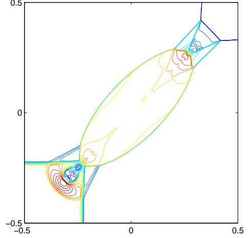
Figure 4.9: [S_{12}^+ J_{23}^- J_{34}^+ S_{41}^-] . The initial data are \rho_1 = 1.4, u_1 = -4.125, v_1 = -4.125, p_1 = 1.0 ; \rho_2 = 8.0, u_2 = 4.125, v_2 = -4.125, p_2 = 116.5 ; \rho_3 = 20.0, u_3 = -4.125, v_3 = -4.125, p_3 = 116.5 ; \rho_4 = 8.0, u_4 = -4.125, v_4 = 4.125, p_4 = 116.5 . The meshes are 200 \times 200 . The output time is t = 0.055 . The monitor function is \omega = \sqrt{1 + |\nabla u|^2 + |\nabla v|^2 + 5|\nabla \rho|^2} .
