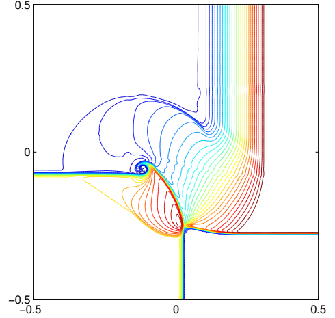
Figure 4.21: [R_{12}^+ J_{23}^+ J_{34}^+ S_{41}^+] . The initial data are \rho_1 = 1.0, u_1=0.1, v_1=-0.3, p_1=1.0 ; \rho_2=0.5179, u_2=-0.6259, v_2=-0.3, p_2=0.4 ; \rho_3=0.8, u_3=0.1, v_3=-0.3, p_3=0.4 ; \rho_4=0.5313, u_4=0.1, v_4=0.4276, p_4=0.4 . The mesh cells are 300 \times 300 . The output time is t = 0.2 . The monitor function is \omega = \sqrt{1+1.0(|\bar{\nabla}u|^2+|\bar{\nabla}v|^2+|\bar{\nabla}\rho|^2)} .
