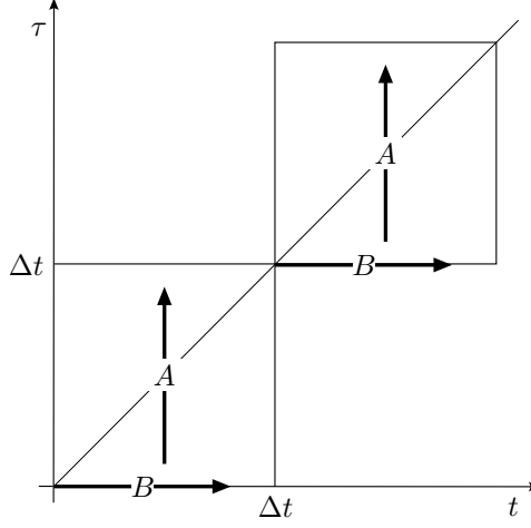
FIGURE 1. A schematic view of Godunov splitting.
