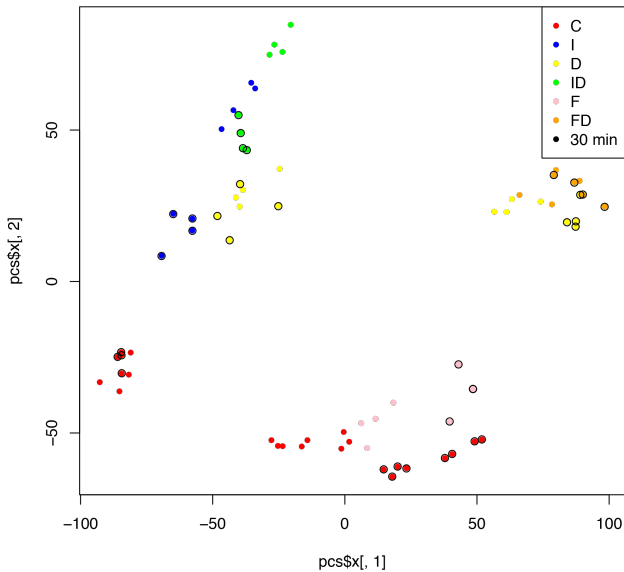
Figure 6: PCA for quality control
