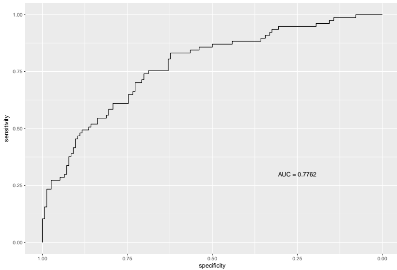
ROC curve
