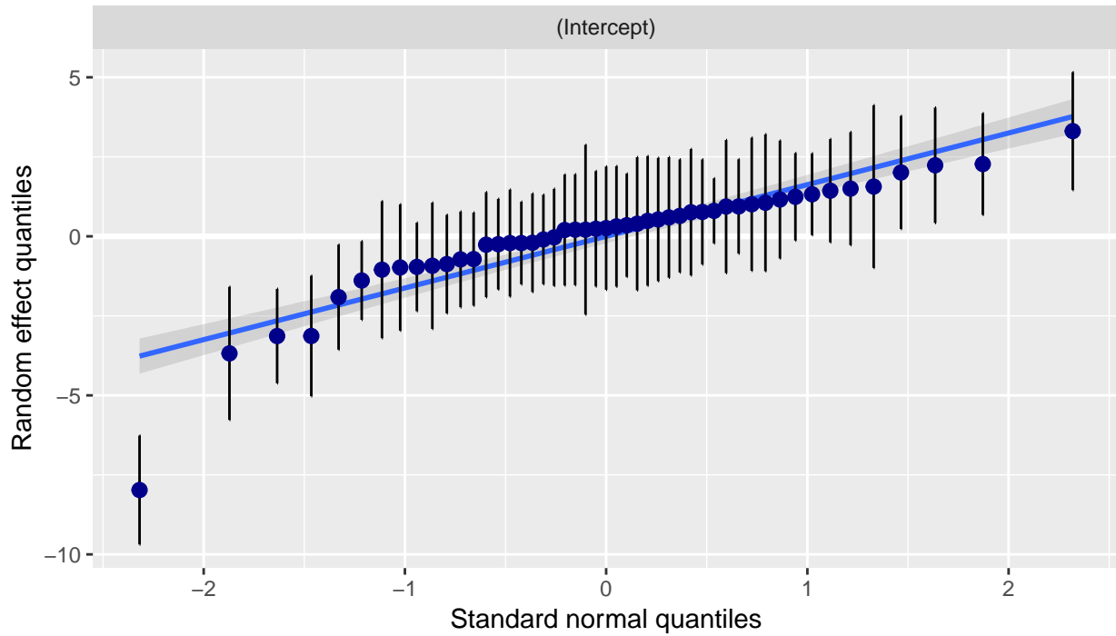
QQ-plot of random intercepts
