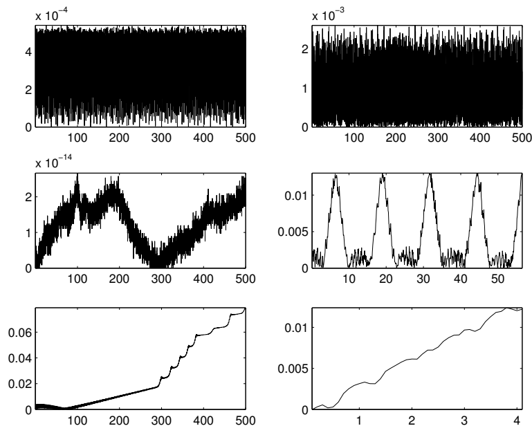
Figure 1: Density (left column) and energy along (SMEXP), (L1) and (PASSA) (from the top to the bottom) for the initial condition (18). Number of Fourier modes M = 512 , time step 0.1.
