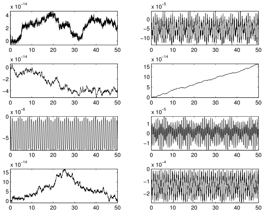
Figure 3: Density (left column) and energy along (SPMEXP-D), (SPMEXP-DE), (MULTI) and (B) (from the top to the bottom) for the initial condition (18). Number of Fourier modes M = 512 , time step 0.025.
