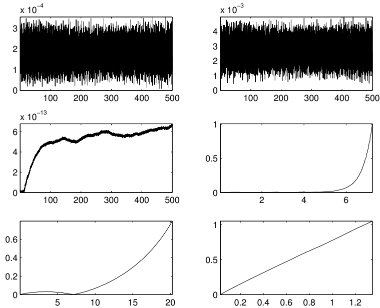
Figure 2: Density (left column) and energy along (SMEXP), (L1) and (PASSA) (from the top to the bottom) for the initial condition (19). Number of Fourier modes M = 512 , time step 0.025.
